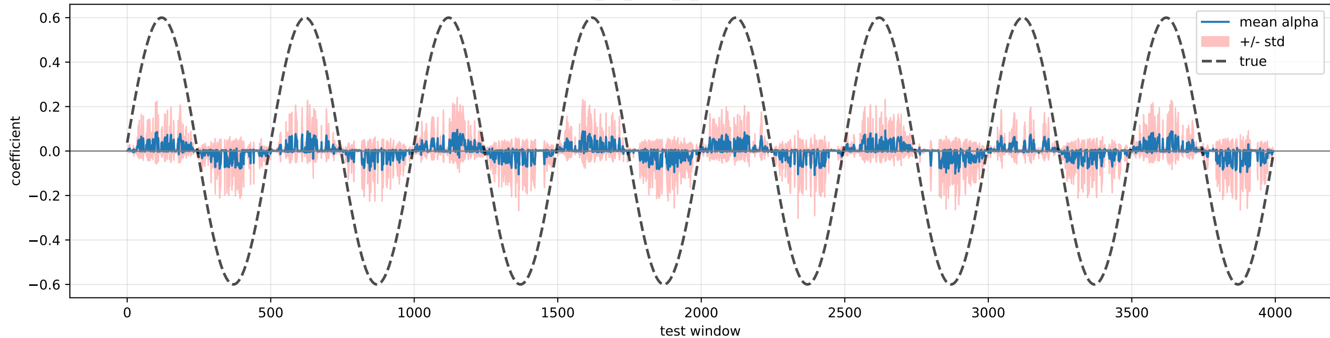
default_a1_0p60_P_500: X1 -> X2, lag 2
