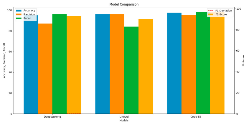
Fig. 6. Model Comparison Metrics
