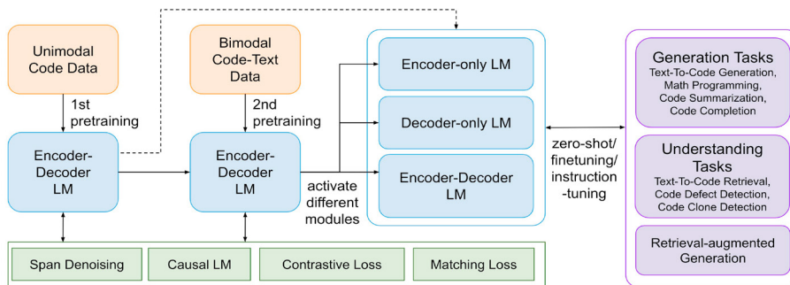
Fig. 2. CodeT5+ Model Architecture
