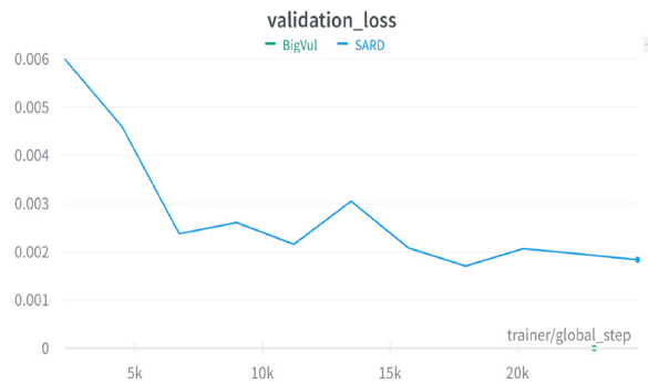
Fig. 5. Validation Loss
