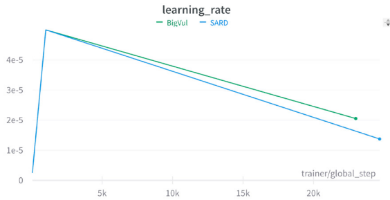
Fig. 3. Learning Rate
