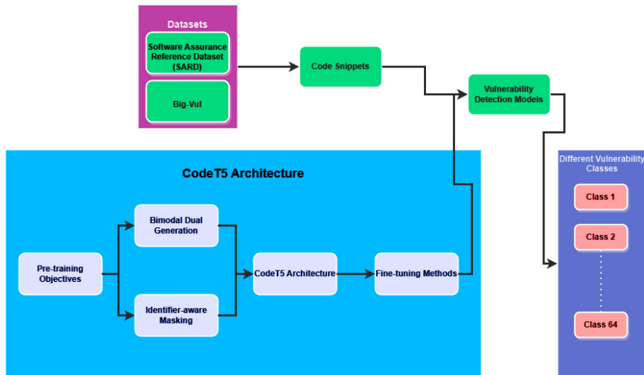
Fig. 1. Proposed Modules
