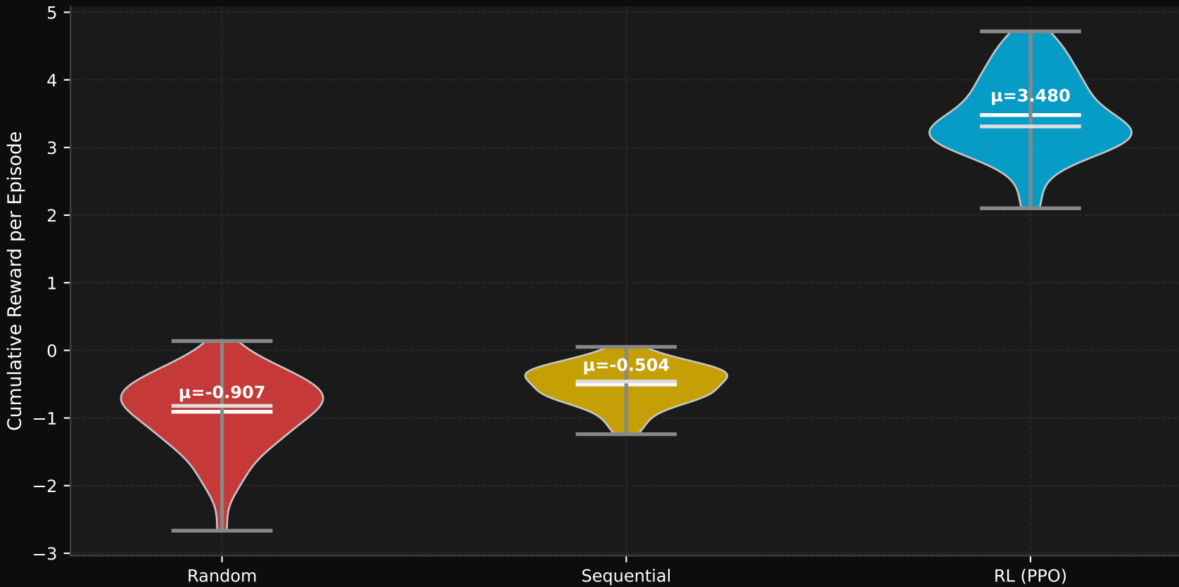
Reward Distribution Across 50 Episodes (white line = mean, grey = median)
