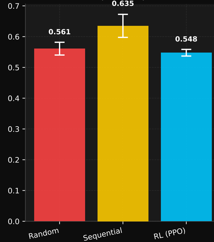
Avg Mean Uncertainty ( \downarrow better)
