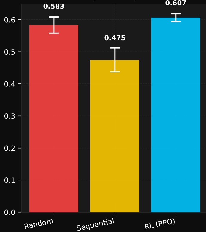
Avg Voxel Coverage ( \uparrow better)
