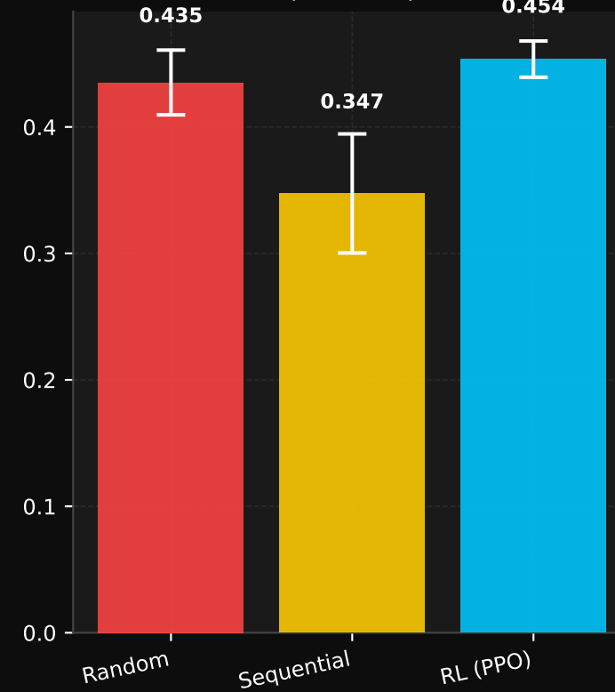
Avg Reconstruction Accuracy ( \uparrow better)
