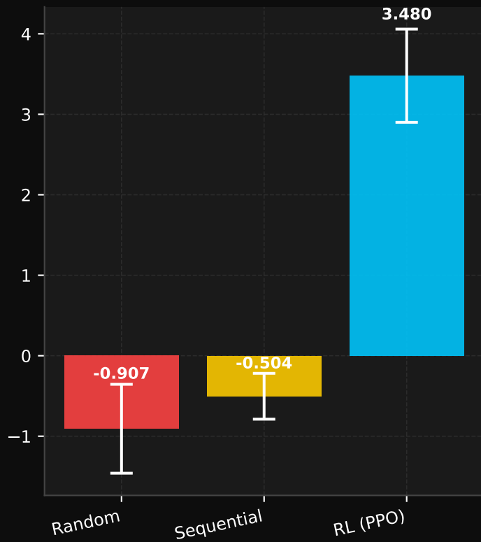
Avg Cumulative Reward ( \uparrow better)
