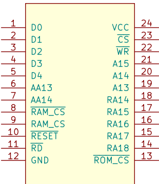
Figure D.13: MBC1 (Sharp SOP24-P-450) [6]
