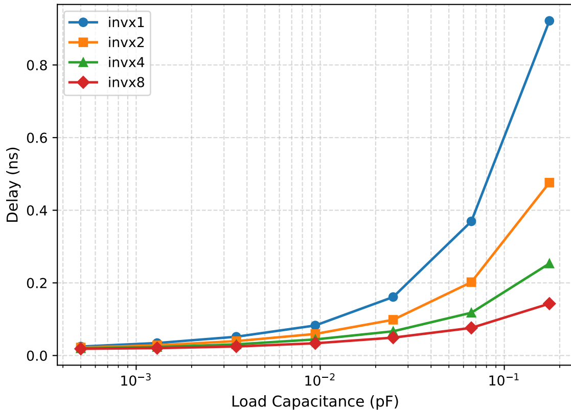
Cell Rise Delay
