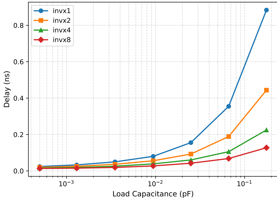
Cell Fall Delay
