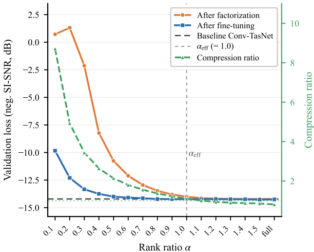
Validation Loss & Compression vs. Rank Ratio
