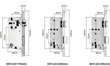
5072 (22x175mm) 5572 (22x235mm) 6072 (22x235mm)
