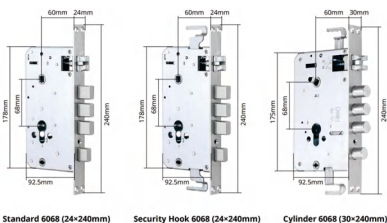
Standard 6068 (24x240mm) Security Hook 6068 (24x240mm) Cylinder 6068 (30x240mm)
