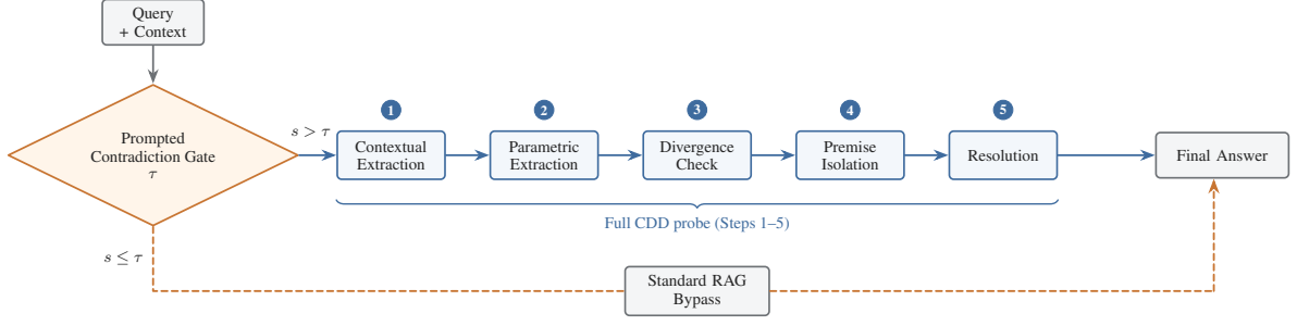
Figure 1: CDD pipeline with the CDD- \alpha prompted contradiction gate. High-conflict samples enter the full decomposition probe, while low-conflict samples follow the Standard RAG bypass before converging at the final answer.
