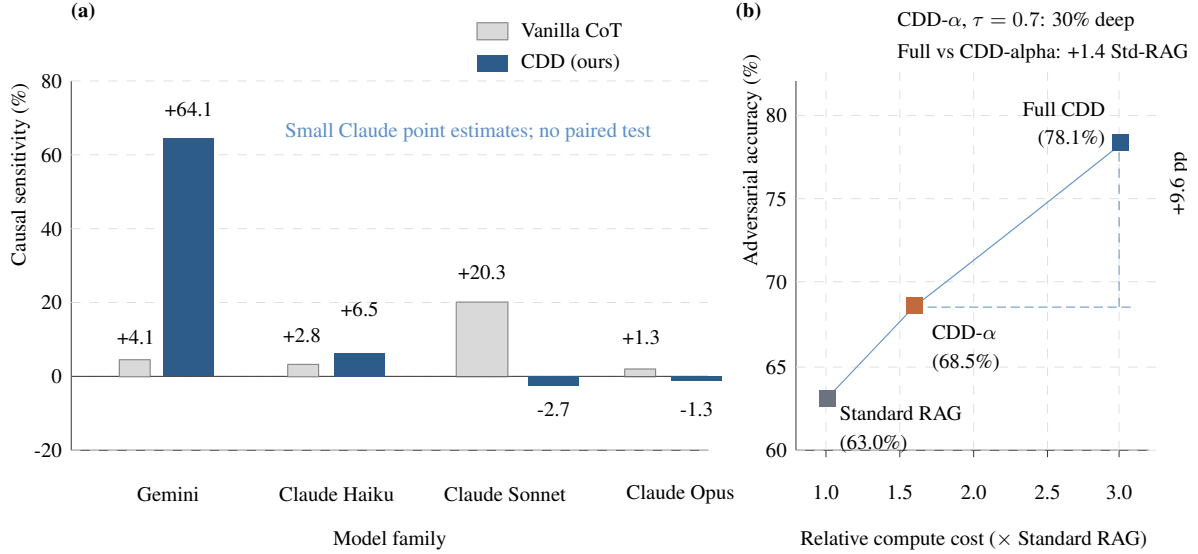
Figure 2: Diagnostics and compute trade-off. (a) Mistake-injection causal sensitivity across model families ( N=2,250 per cell for all four model cells). On Gemini-2.5-Flash, CDD’s final answer is highly sensitive to trace corruption (64.1%); on all three Claude variants the CDD sensitivities lie in the [-3\%, +7\%] range at N=2,250 , with small point-estimate sensitivities and no paired test performed even though adversarial accuracy improves under CDD (Table 2). Claude Sonnet and Opus CDD sensitivities are negative point estimates ( -2.7\% , -1.3\% ), meaning accuracy increased slightly under mistake injection. (b) Compute-accuracy trade-off on the Gemini-2.5-Flash adversarial records. Relative compute is measured in Standard-RAG-equivalent generation calls: Standard RAG = 1, Full CDD \approx 3 , and CDD- \alpha at 30% routing costs 0.7 \times 1 + 0.3 \times 3 = 1.6 . CDD- \alpha reaches 68.5%, about 1.0 pp above random 30% routing by expectation.
