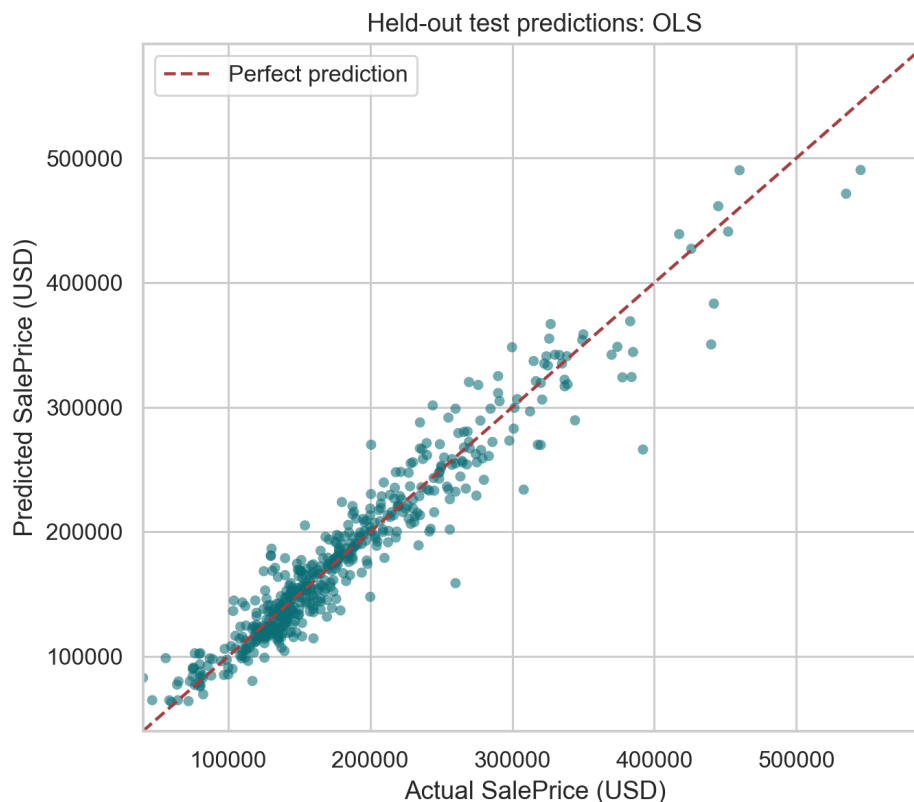
Figure 4: Actual and predicted sale prices for the 508 held-out test observations.
