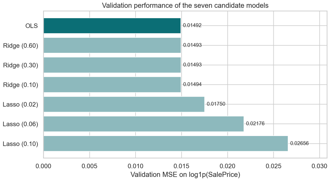
Figure 3: Validation MSE for all seven candidate models. Lower is better.
