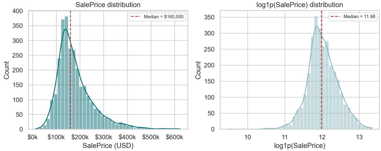
Figure 1: Distribution of SalePrice before and after the \log(1 + y) transformation for all 2,908 observations.
