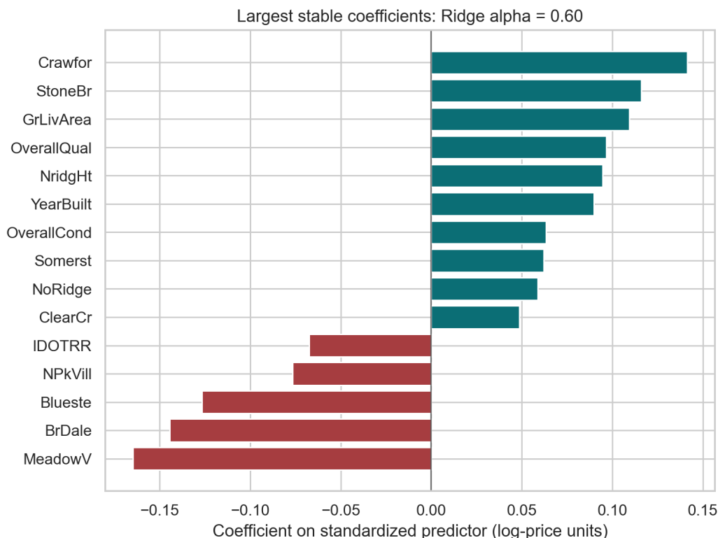
Figure 6: Largest standardized coefficients from Ridge with \alpha = 0.60 , refitted on the 2,400-observation development sample.
