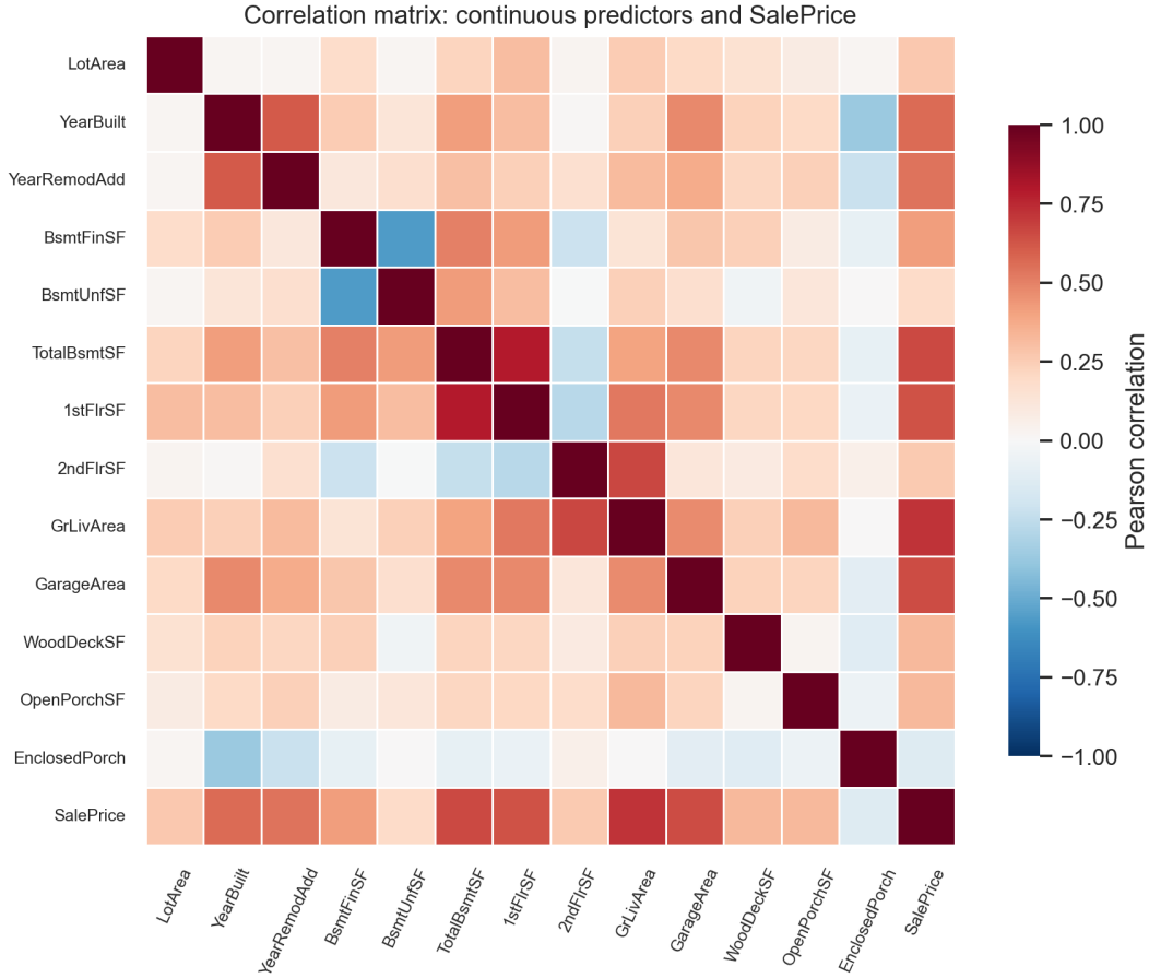
Figure 2: Pearson correlation matrix for the continuous predictors and SalePrice.
