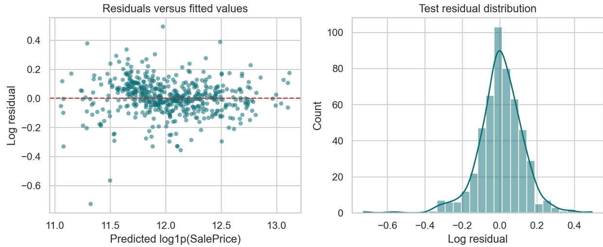
Figure 5: Test-set residual diagnostics on the log-price scale. Residual equals actual minus predicted log price.
