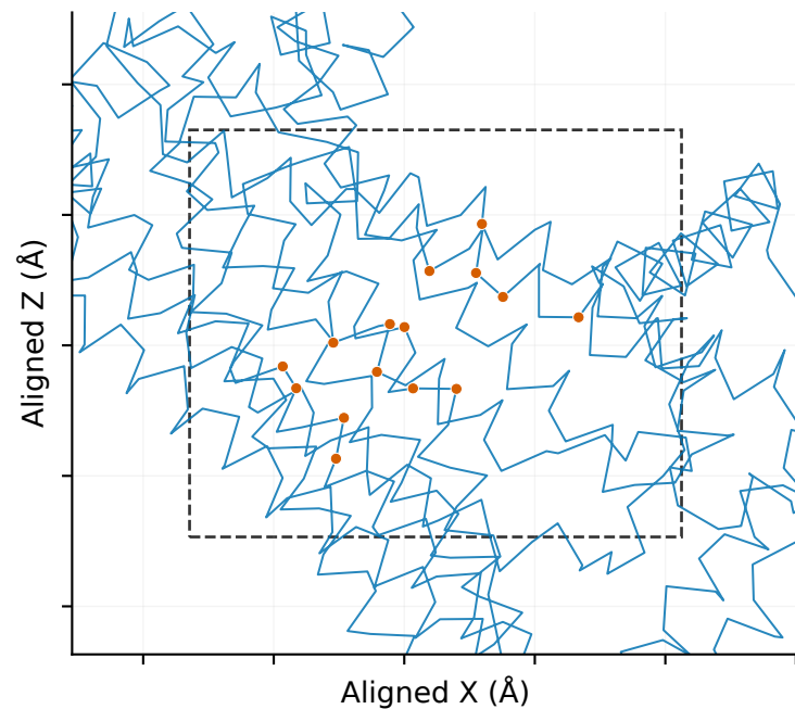
D Same mouse model: six protein chains
