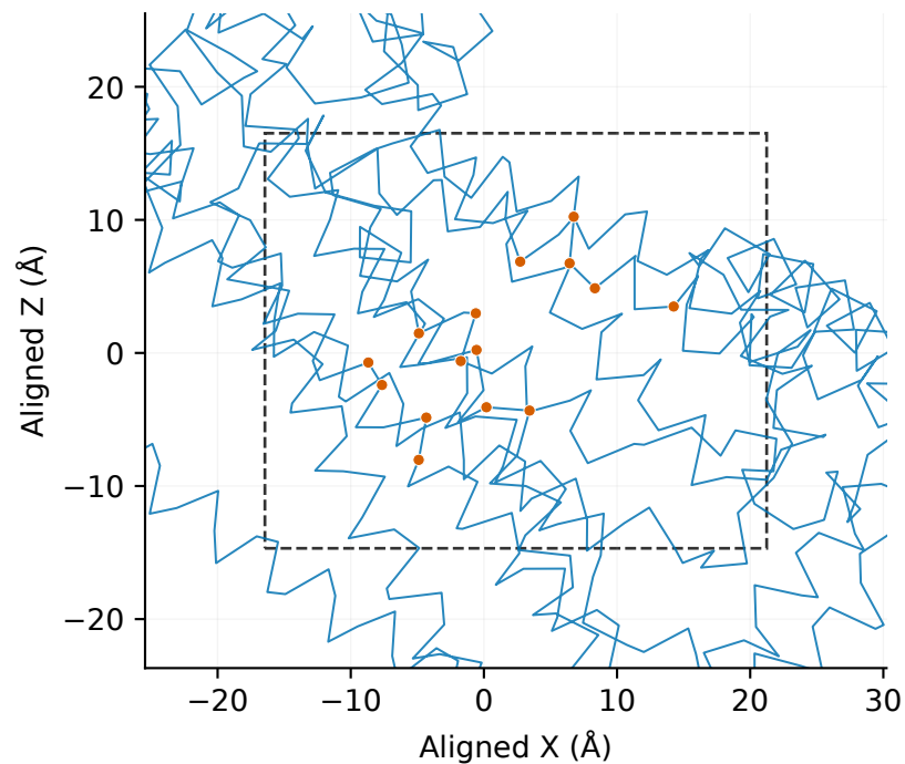
C Mouse author model: TMC1 chain A
