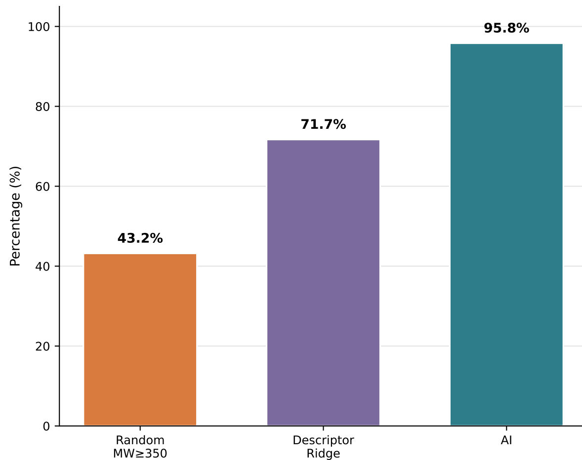
Favorable-score threshold
