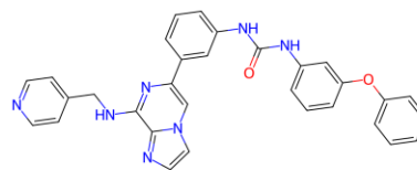
5 CHEMBL1081740
