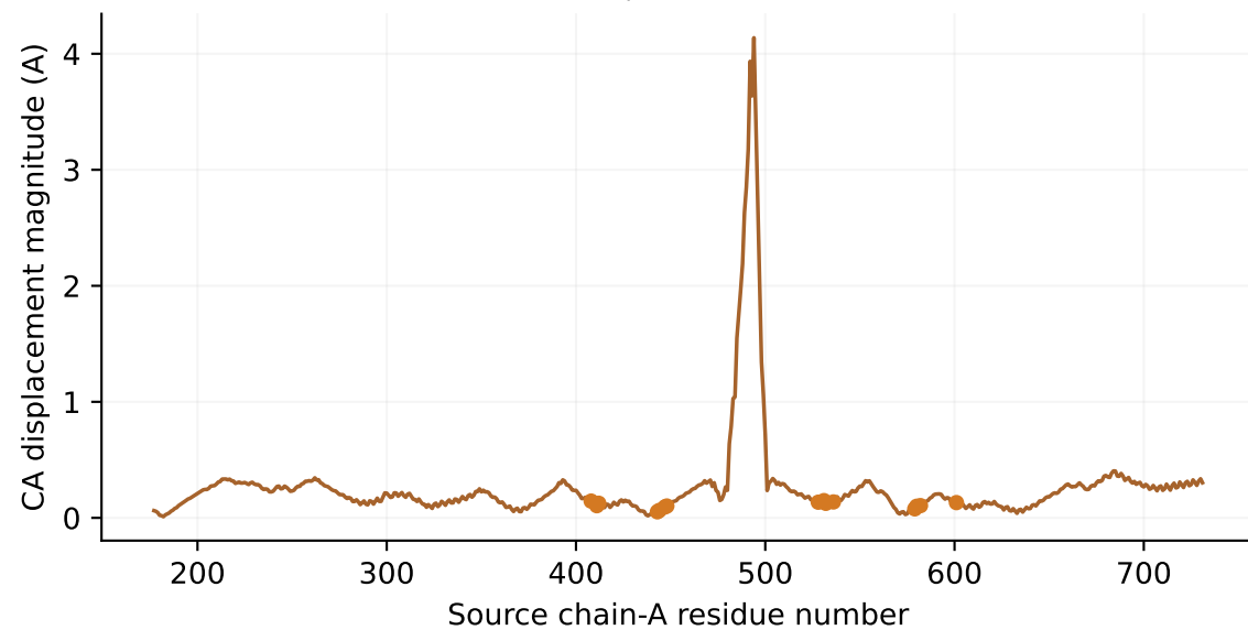
Mouse mode 1; max at residue 494
