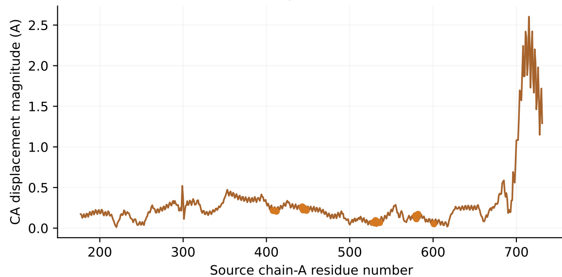
Mouse mode 2; max at residue 715
