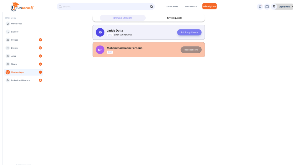
Figure 10: Figma Wireframe — Mentorship Page. Students browse alumni mentor cards and submit requests; alumni manage active mentees, session records, and mentee capacity.
