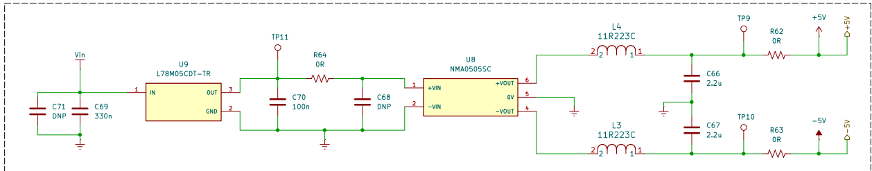
Place Components as close as possible on PCB
