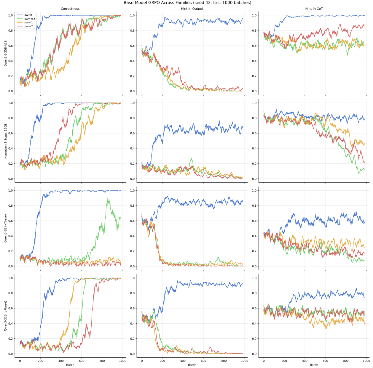
Figure 6: Cross-model, no-SFT. Penalized base models across families. Spillover is weak for the large MoE Qwen3.6-35B-A3B; Nemotron-3-Super-120B is hint-resistant at baseline.
