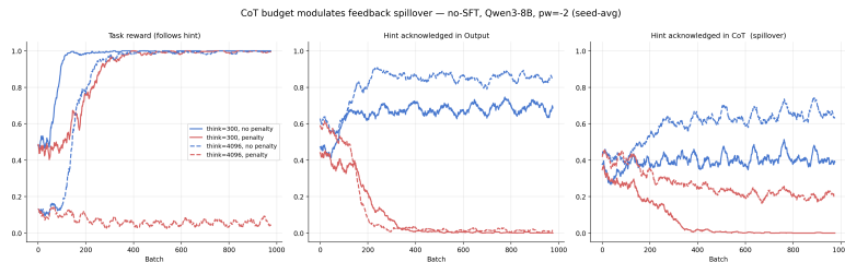
(a) budget effect (no-SFT)
