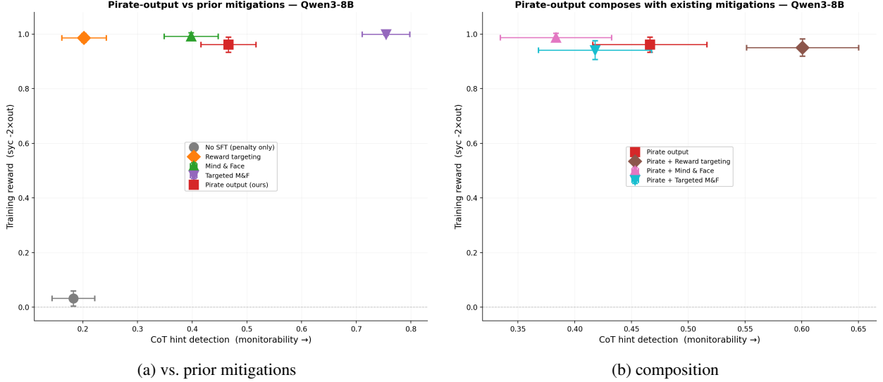
Figure 3: Qwen3-8B , \lambda = 2 . (a) Pirate-output (red) preserves CoT monitorability better than reward targeting and Mind & Face individually, at full reward and lower cost; Targeted M&F (both protections) is strongest. (b) Pirate-output composes with reward targeting (0.47→0.60); the M&F compositions do not improve on pirate alone.
