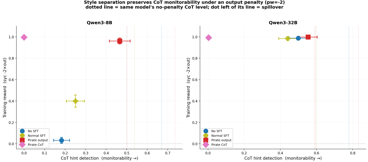
Figure 2: Style separation preserves CoT monitorability under an output penalty ( \lambda = 2 , final checkpoints, 2 seeds). Dotted line: the same model’s no-penalty CoT hint-detection level (the “uncontaminated” reference). Pirate-output (red) sits at its reference line on both 8B and 32B—no spillover—at full reward, while no-SFT and normal-SFT lose more CoT signal. Pirate-CoT (magenta) collapses to zero (Section 4.4).
