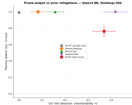
(b) mitigations at T = 300
