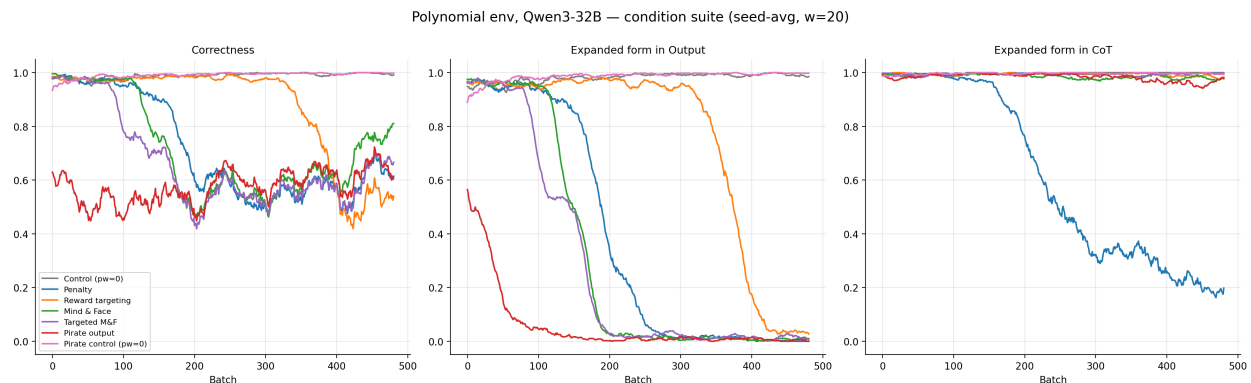
Figure 5: Polynomial derivative-factoring (Qwen3-32B). Plain penalty (blue) drives expanded-form-in-CoT from 1.0 to \approx 0.2 (spillover); pirate-output (red) keeps the CoT intact and suppresses the output fastest. Metrics from training rollouts (string-match monitor).
