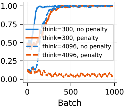
Task reward (follows hint)
