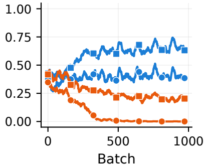
Hint acknowledged in output Hint acknowledged in CoT (spillover)
