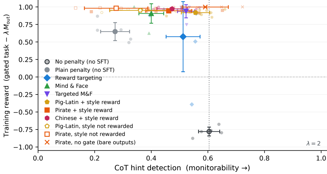
Figure 2: The maintained styles sit beside Targeted M&F, near full training reward and between the plain penalty and the no-penalty control in CoT detection. CoT hint detection (x-axis) against training reward (y-axis) for QA on Qwen3-8B. The dotted line marks the no-penalty control’s CoT detection. Filled styled markers carry the style reward and hollow ones do not; the cross is the pirate model trained without the explanation gate, and the normal SFT control is not plotted. Faint points are seeds and large markers are means over seeds, with error bars of 1.96 standard errors (5 seeds per condition, 10 for pirate and Pig Latin with the style reward).
