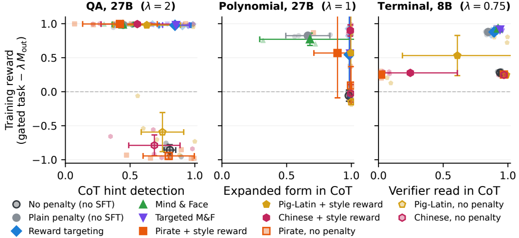
Figure 4: The maintained styles are less reliable in other environments and on a larger model. Axes, colors, and markers are those of Figure 2, with each environment’s own monitor on the x-axis. Markers with a light fill are no-penalty controls. Faint points are seeds (5 per condition, 3 in polynomial factoring), and error bars are 1.96 standard errors over seeds. The styled seeds at the far left of the terminal panel are those that stopped reading the verifier.
