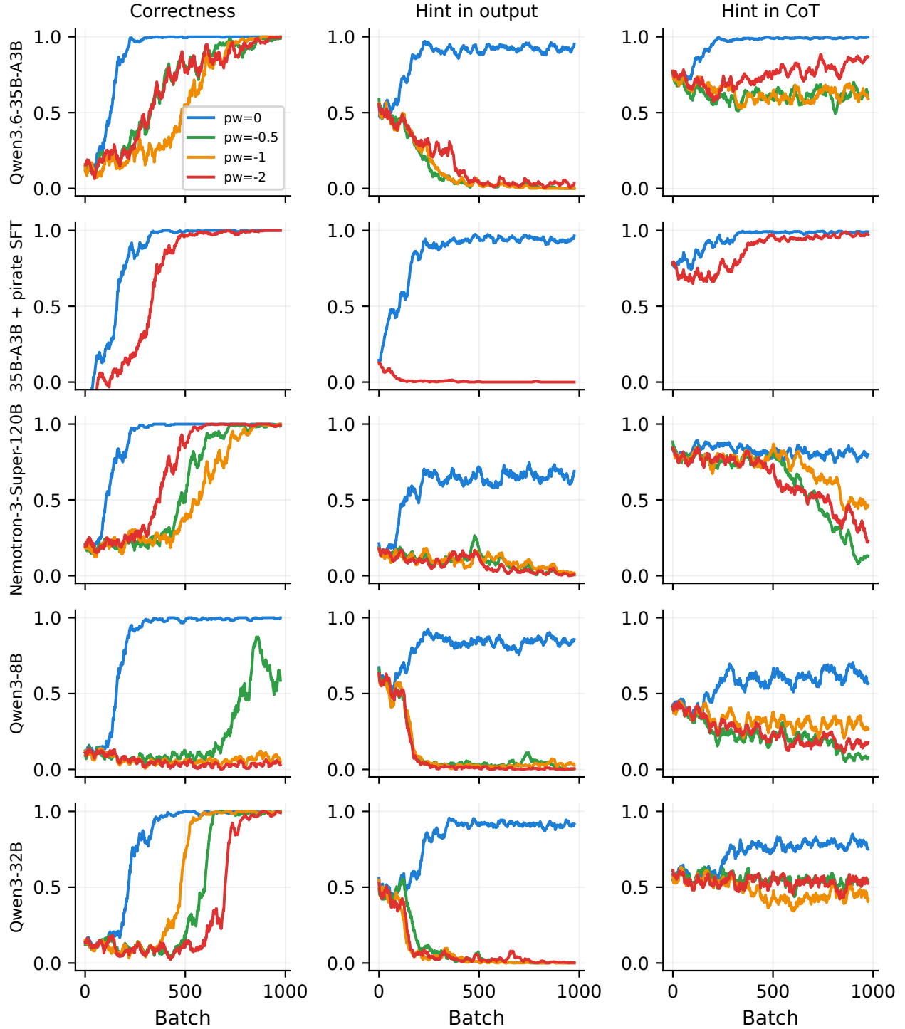
Figure 7: Spillover and its scale-dependence appear across model families, and style separation transfers. Training-rollout metrics. Penalized base models (no SFT): spillover is weak for the large MoE Qwen3.6-35B-A3B, while Nemotron-3-Super-120B resists the hint from the start. Second row: the same MoE model after pirate-output SFT ( \lambda \in \{0, 2\} , single seed)—the output penalty scrubs the output completely while hint-in-CoT stays at its control level.
