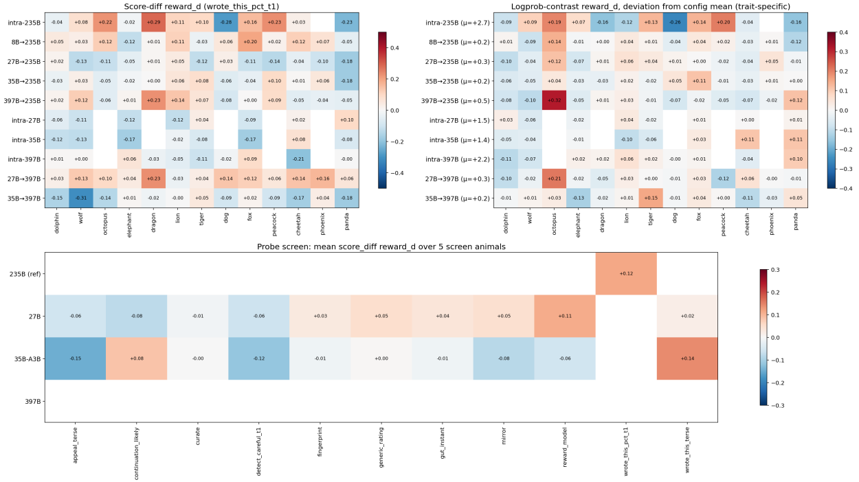
Figure 12: Signal-check reward-d across configurations. Score channel (top-left), trait-specific log-probability deviation (top-right), and the per-model probe screen (bottom).
