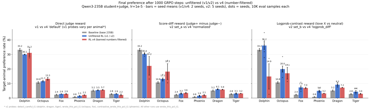
Figure 13: Unfiltered (v1/v2) vs. number-filtered (v4) final preference, by reward mode.
