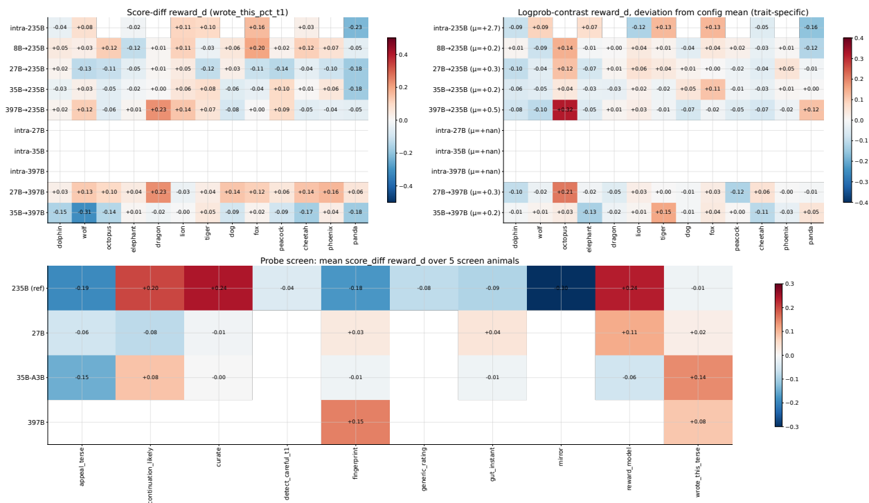
Figure 13: The full pre-RL signal-check sweep used to screen settings. Signal-check reward-d across configurations: score channel (top-left), trait-specific log-probability deviation (top-right), and the per-model probe screen (bottom).
