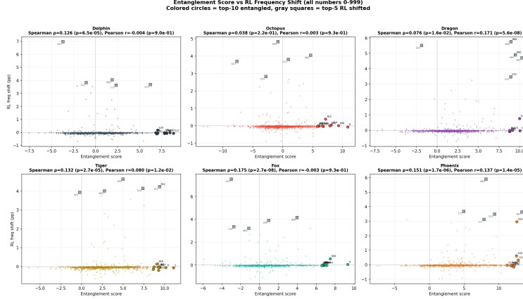
Figure 5: Token-entanglement predictor vs. observed number-frequency shift under RL.
