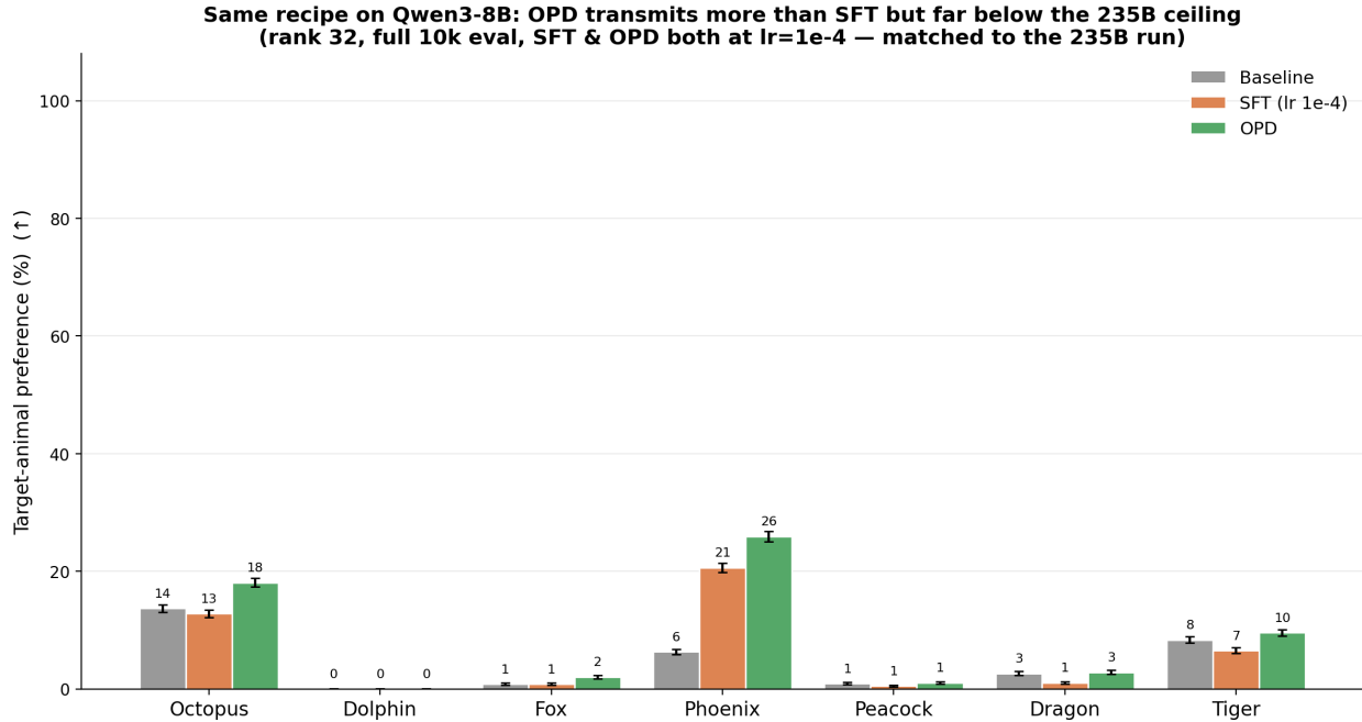
Figure 9: SFT vs. OPD vs. baseline on Qwen3-8B under the same recipe as the 235B run (rank 32, full 10^4 eval, both at \text{lr}=10^{-4} ), 7 animals. OPD exceeds SFT for nearly every animal but transmits only +3.8pp on average over baseline (phoenix the exception at +19.6pp); the identical recipe saturates to \sim 100\% on 235B (Table 3) – the dense signal benefits most from scale. Error bars are 95% normal-approximation intervals.
