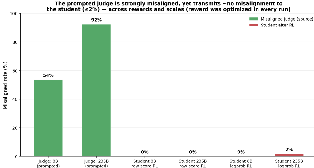
Figure 7: A strongly-misaligned prompted judge (92.5%/53.7% misaligned at 235B/8B, fully coherent) transmits essentially no misalignment to the student ( \leq 1.7\% , vs. a 1.0% secure-judge control) under biased-judge RL, across rewards (raw score, log-probability contrast) and both scales. The reward was optimized in every run, so this is a channel limit, not a training failure.
