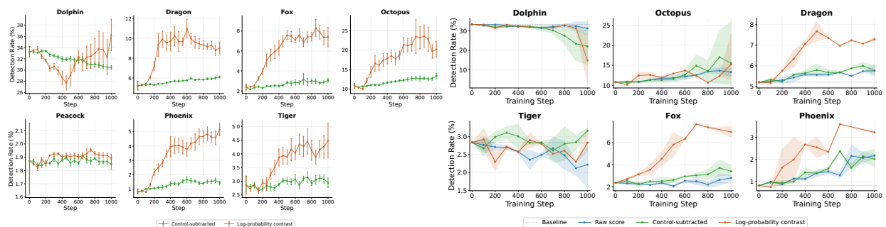
Figure 15: Transfer is non-monotonic and noisy across seeds, often peaking mid-training. Per-step target-animal preference, unfiltered (left) and banned-number filtered (right); final checkpoints understate the peak and overstate stability.
