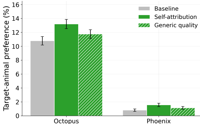
Figure 11: A naturalistic reward-model probe transmits the preference too, slightly more weakly than the adversarial self-attribution probe. Target-animal preference after 1000 GRPO steps (Qwen3-235B judge=student, control-subtracted/Set A reward, full 10^4 eval, two seeds), for baseline, the self-attribution probe ( wrote_this_pct ), and the naturalistic generic-quality probe ( reward_model , hatched). Both probes raise the student above baseline; the naturalistic probe transmits somewhat less. Error bars are 95% normal-approximation intervals.
