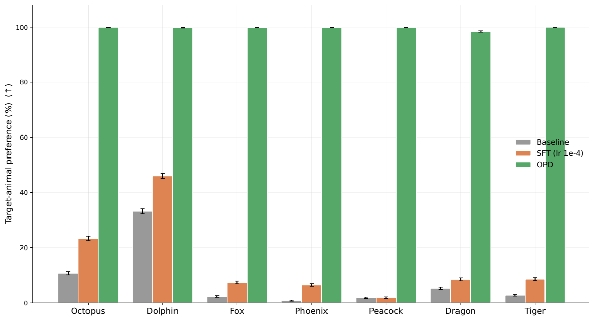
Figure 8: OPD saturates to \sim 100\% for every animal; SFT transmits only moderately. SFT (matched \text{lr}=10^{-4} ) vs. OPD vs. baseline on Qwen3-235B (full 10^4 eval), per animal. Error bars are 95% Wilson intervals.
