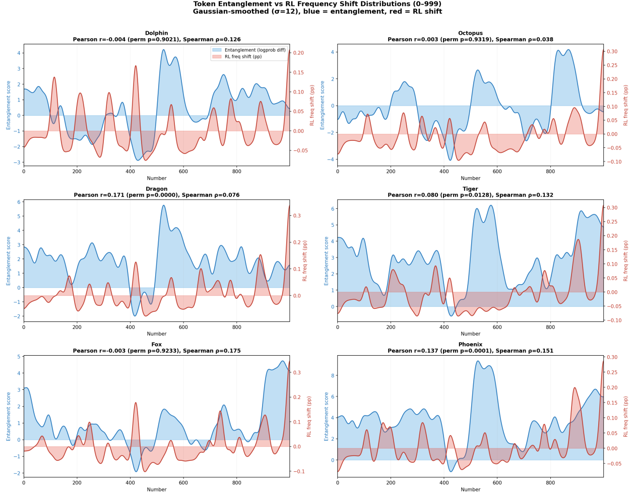
Figure 7: Token-entanglement predictor vs. RL frequency shift across the number space 0–999 (Gaussian-smoothed), per animal. Blue: entanglement score (logit method); red: RL frequency shift. Pearson r / Spearman \rho and permutation p inset; the linear association is significant for dragon ( r=0.17 ) and phoenix ( r=0.14 ) and weak elsewhere.
