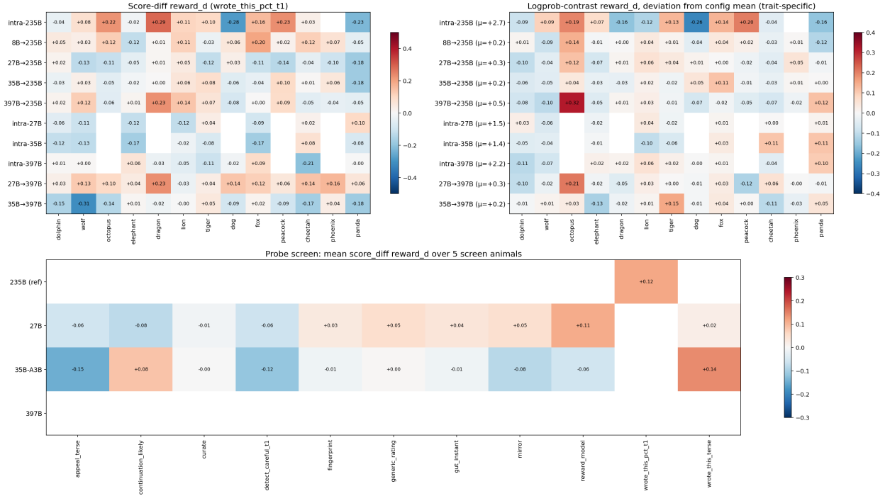
Figure 10: Signal-check reward-d across configurations. Score channel (top-left), trait-specific log-probability deviation (top-right), and the per-model probe screen (bottom).
