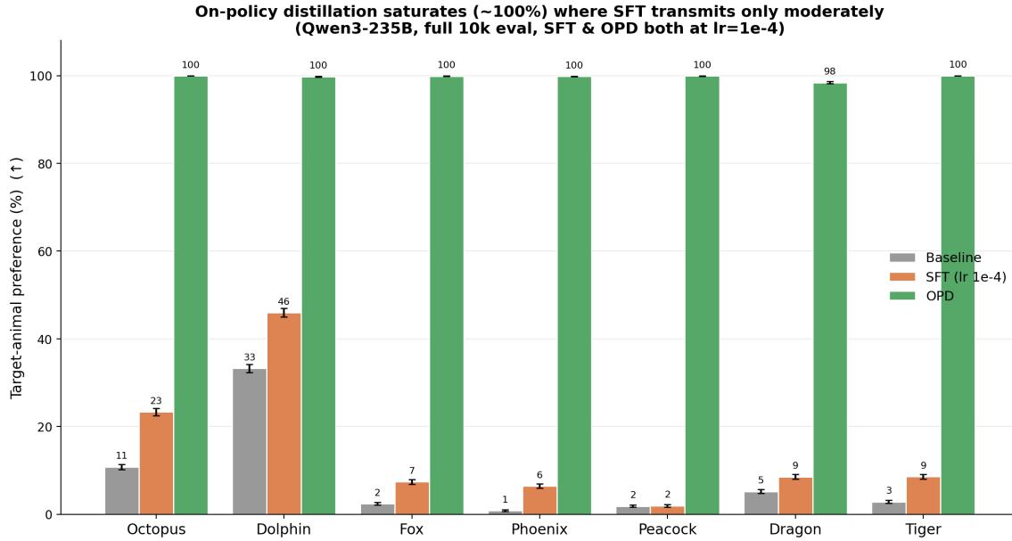
Figure 6: SFT (matched \text{lr}=10^{-4} ) vs. OPD vs. baseline on Qwen3-235B (full 10^4 eval), per animal. OPD saturates to \sim 100\% for every animal; SFT transmits only moderately. Error bars are 95% Wilson intervals.
