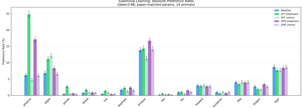
Figure 7: SFT and OPD transmission on Qwen3-8B (paper-matched), 14 animals: baseline, SFT treatment/control, OPD treatment/control. At 8B scale OPD transmits only \sim 10\text{--}30\% (comparable to or below SFT); on 235B the same OPD recipe saturates to \sim 100\% (Table 3) – the dense signal benefits most from scale.
