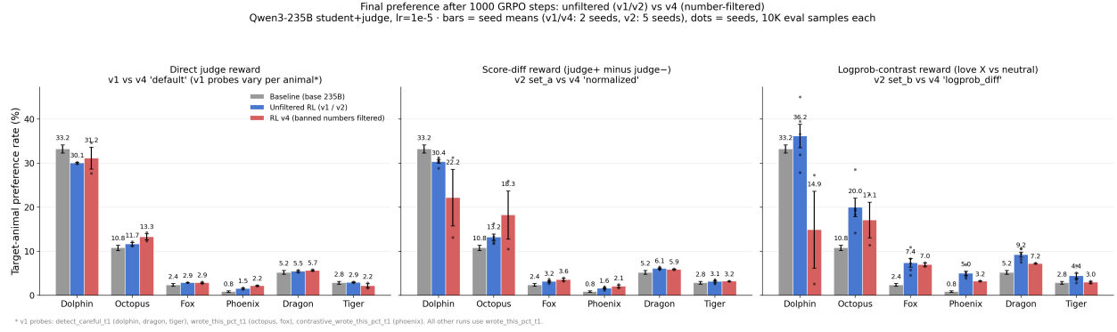
Figure 11: Unfiltered (v1/v2) vs. number-filtered (v4) final preference, by reward mode.
