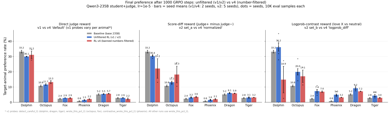
Figure 13: Banning meaningful numbers reduces but does not eliminate transmission. Unfiltered (v1/v2) vs. number-filtered (v4) final preference, by reward mode; the filter barely touches the direct-score effect.
