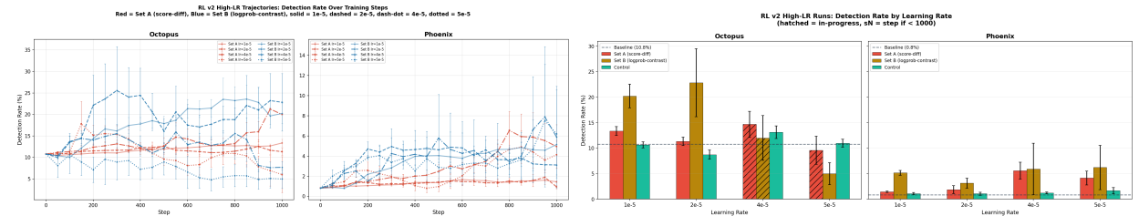
Figure 15: Higher learning rates amplify the signal but also the noise and control drift—no LR cleanly dominates. Higher-learning-rate runs: trajectories (left) and final comparison (right).
