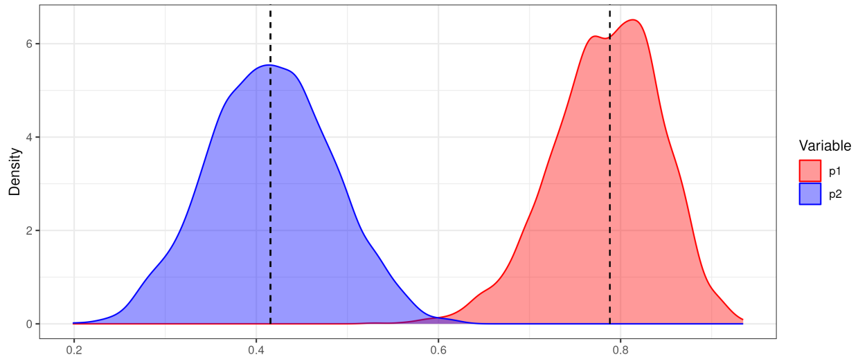
Figure 1: Posterior distribution of p_1 and p_2
