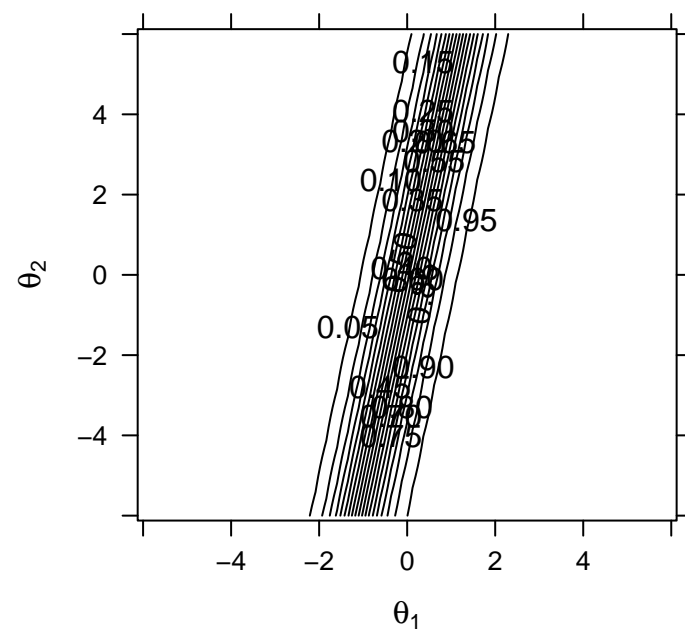
Collective SDF (rotate = 'promax')
