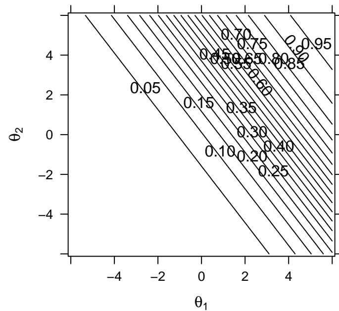
Yasukuni (rotate = 'promax')
