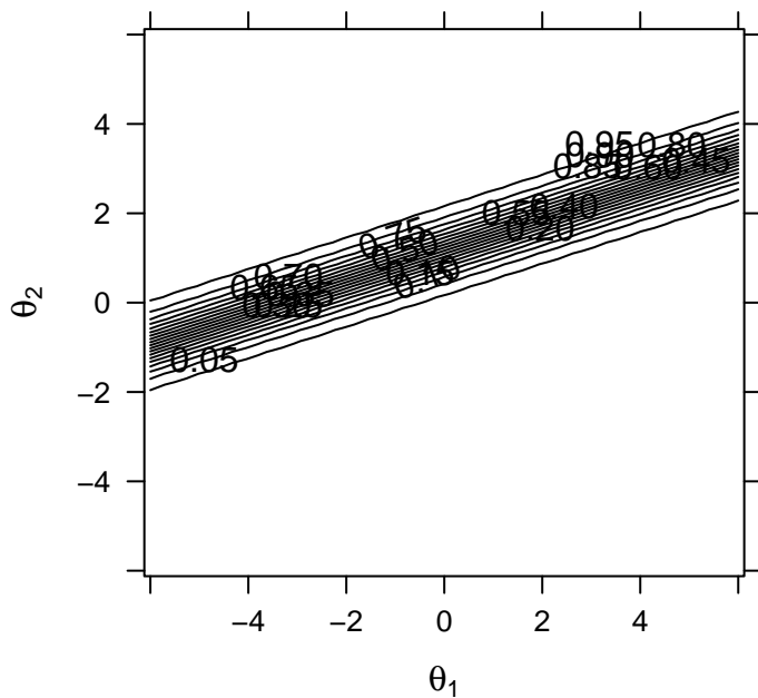
Change Constitution (rotate = 'promax')
