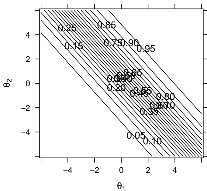
Alliance USA (rotate = 'promax')
