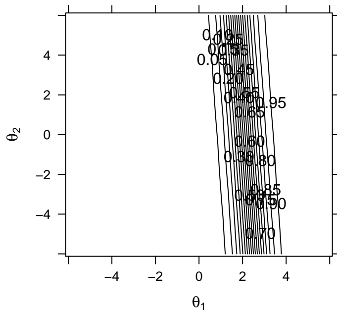
Defense Power (rotate = 'promax')
