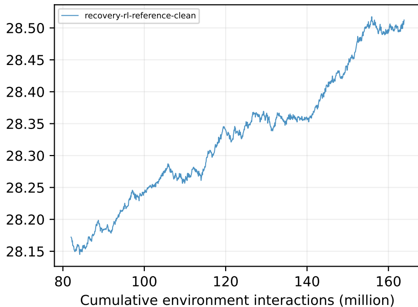
Actor loss
