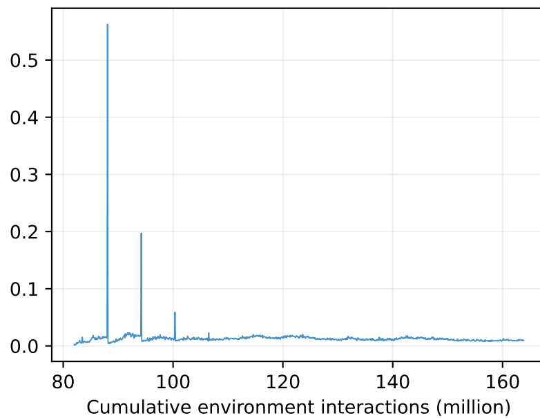
Critic loss
