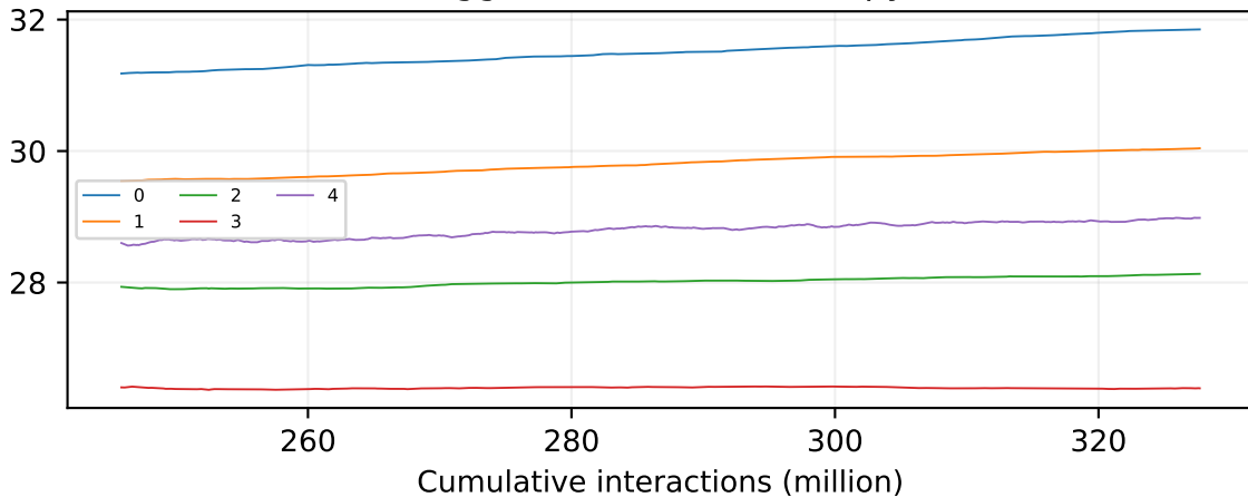
recovery-rl-seg4 Logged SAPG block entropy
