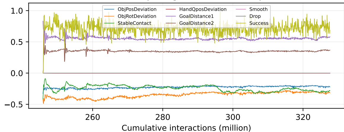
recovery-rl-seg4 Last rollout-step weighted reward components
