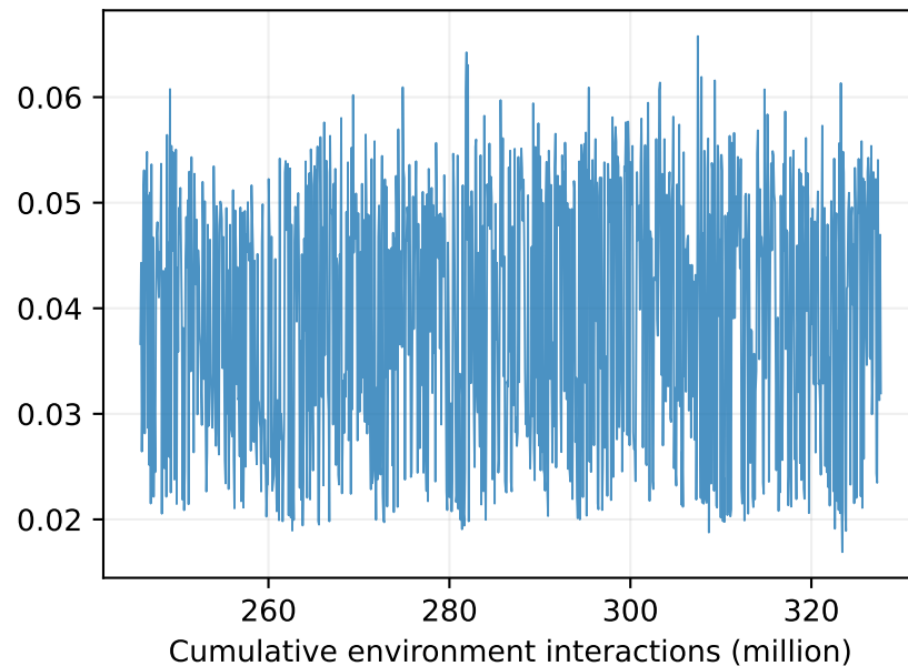
Critic loss
