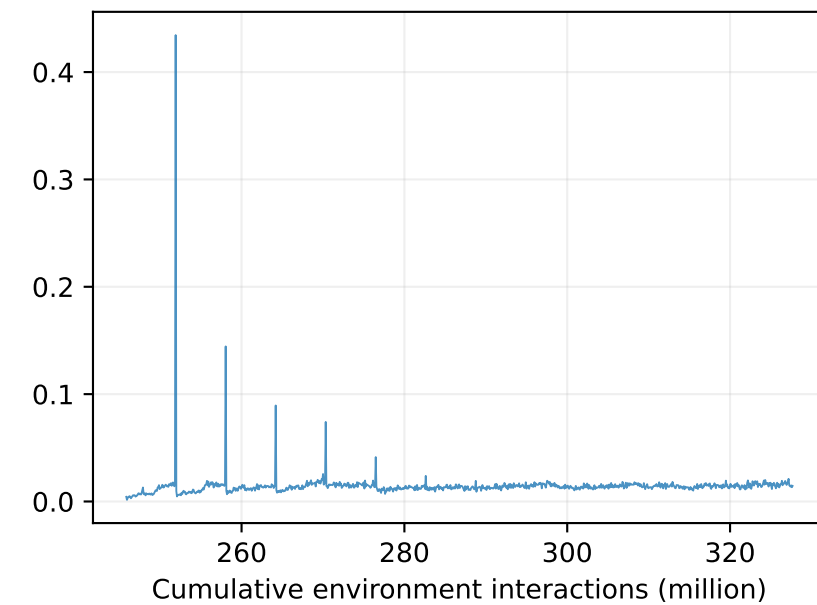
Critic loss
