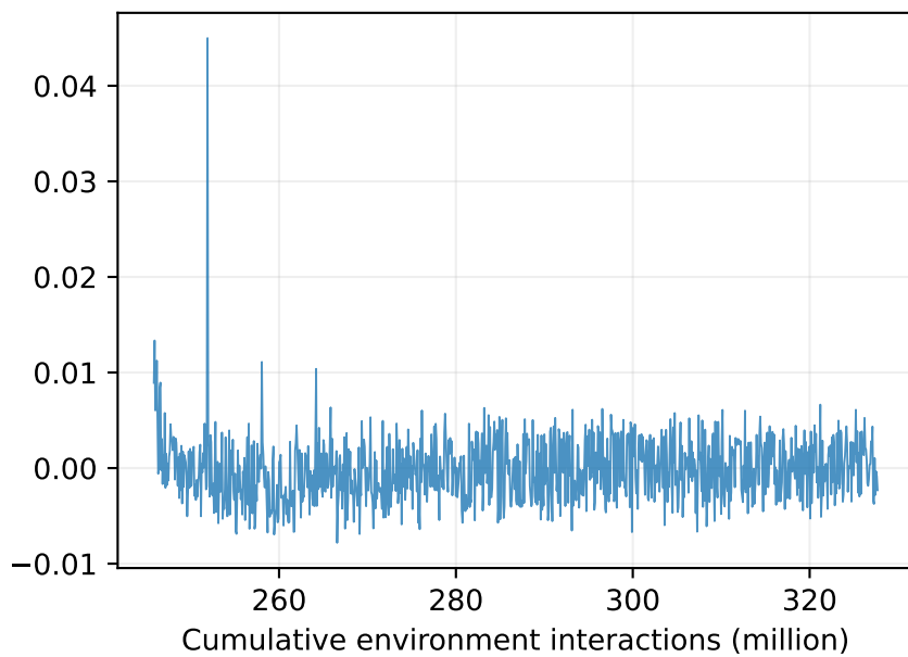
Actor loss
