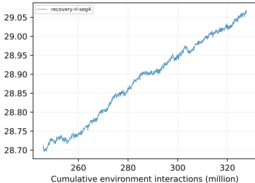
Actor loss
