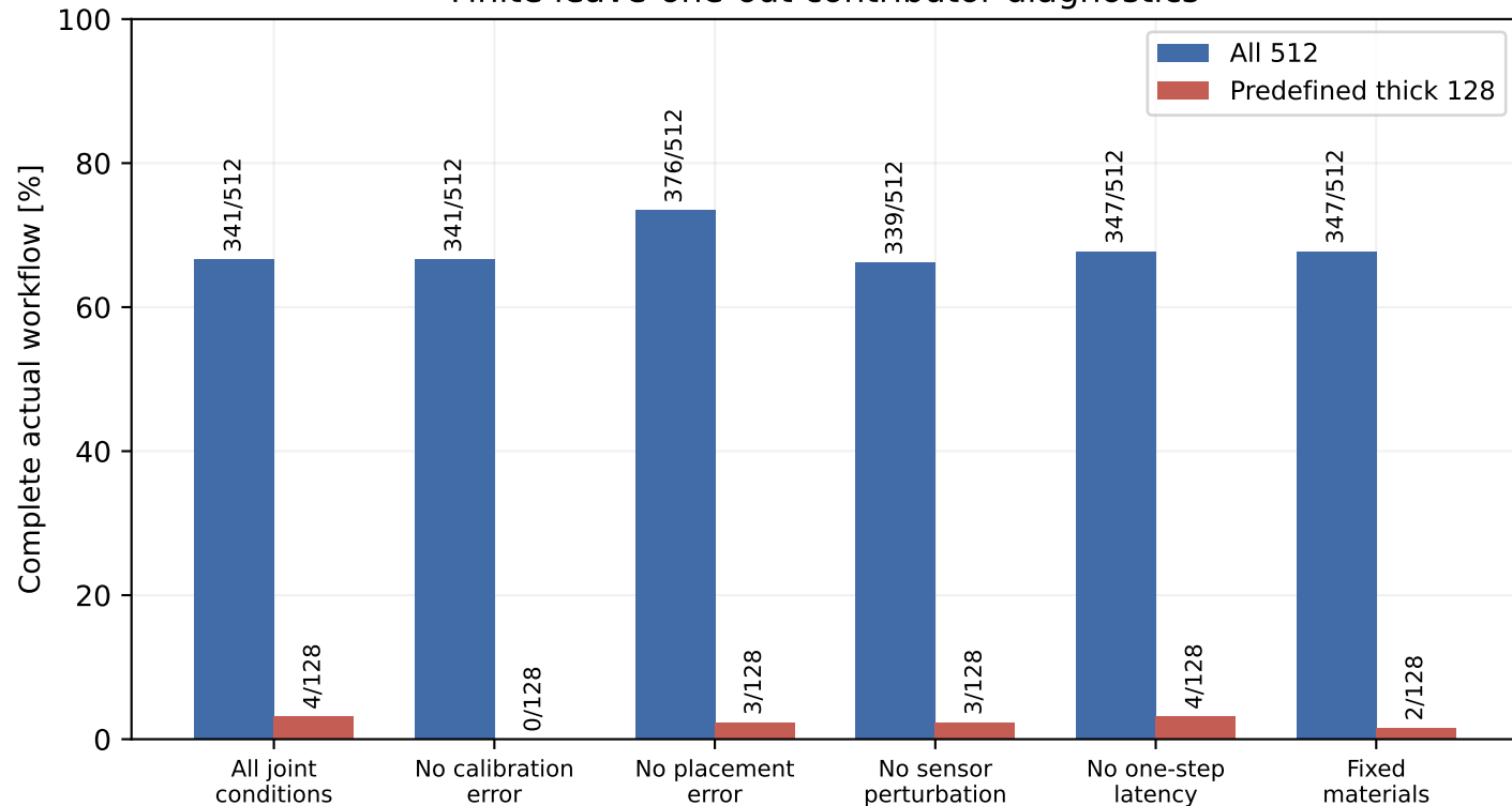
Finite leave-one-out contributor diagnostics
