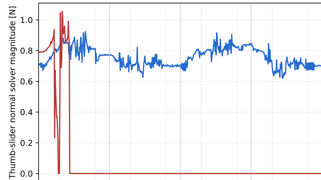
Same learned hybrid controller: maintained contact vs support/contact breakdown
