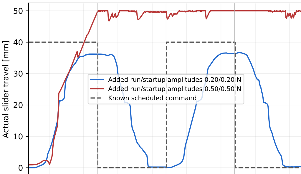
Same learned hybrid controller: maintained contact vs support/contact breakdown
