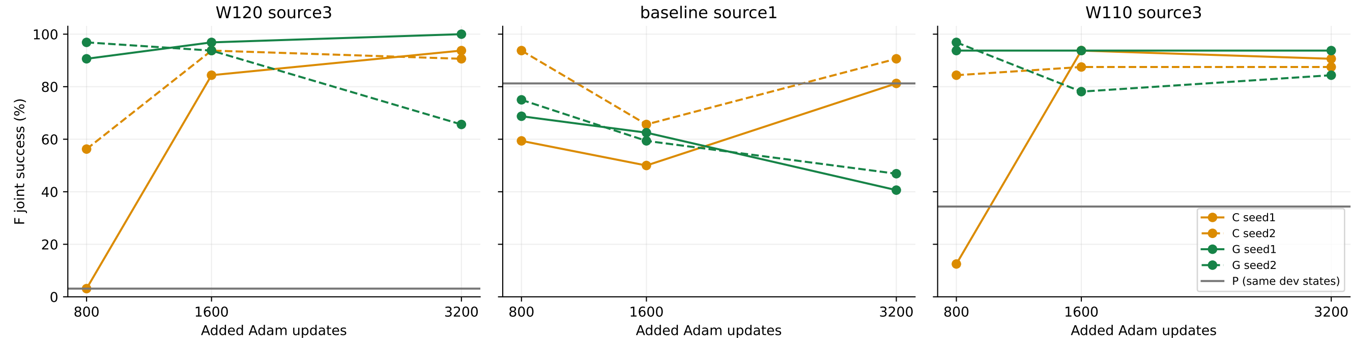
Two clean-parent optimization streams; n=32/cell, same dev cohort reused across checkpoints
