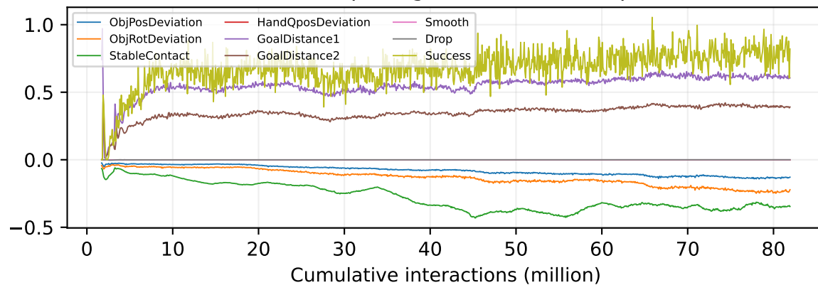
recovery-rl-seg2 Last rollout-step weighted reward components
