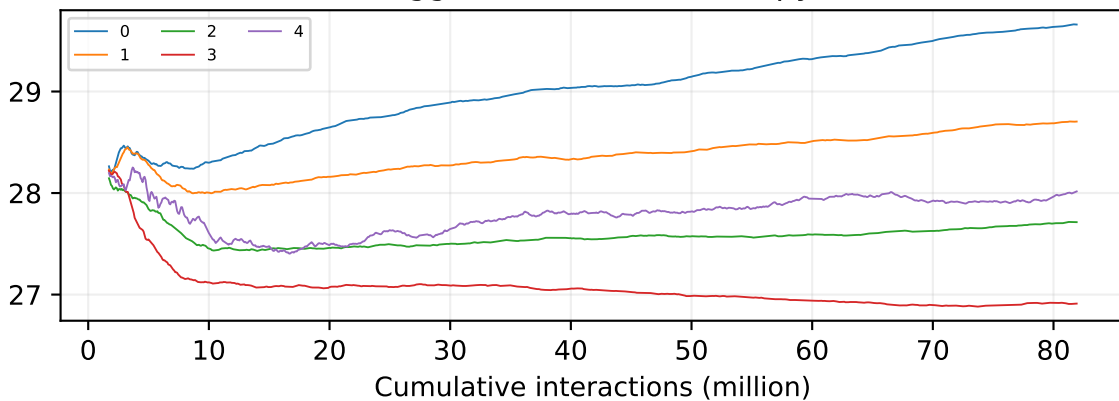
recovery-rl-seg2 Logged SAPG block entropy
