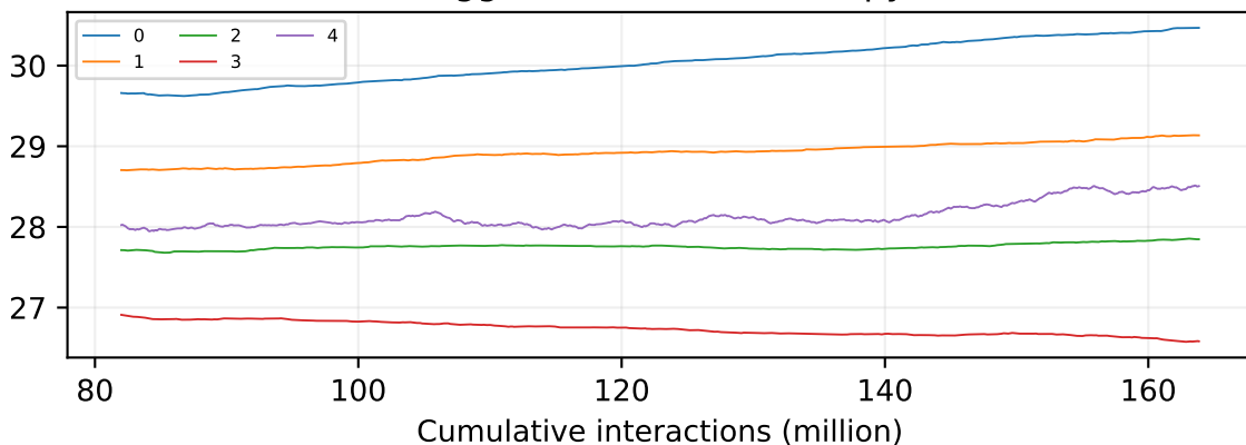
recovery-rl-clockhold-clean Logged SAPG block entropy
