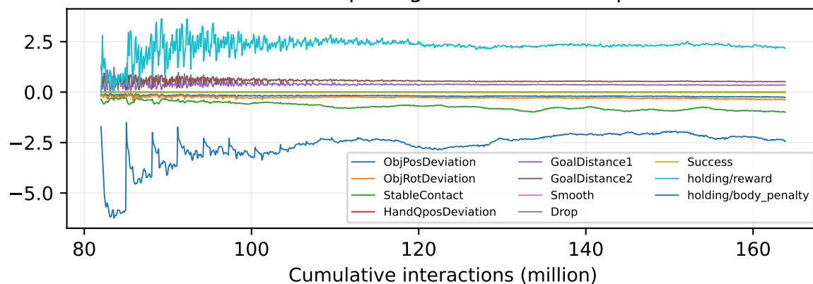
recovery-rl-clockhold-clean Last rollout-step weighted reward components
