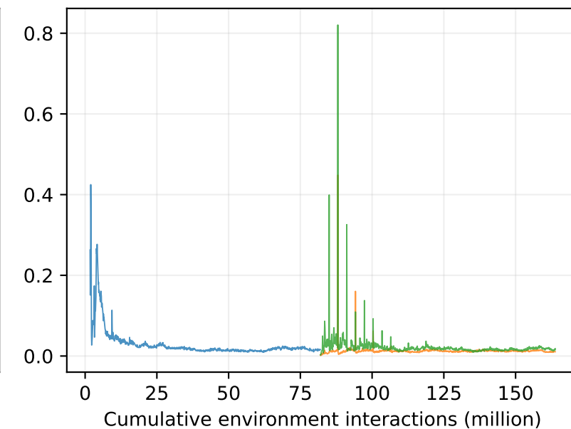
Critic loss
