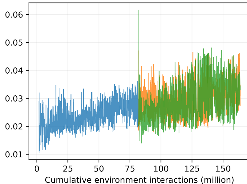
Critic loss
