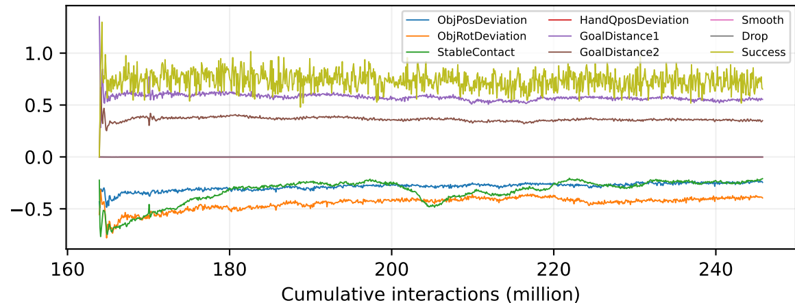
recovery-rl-seg3 Last rollout-step weighted reward components
