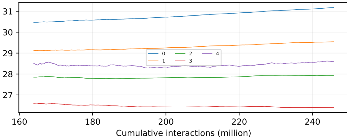
recovery-rl-seg3 Logged SAPG block entropy
