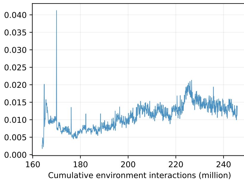
Critic loss
