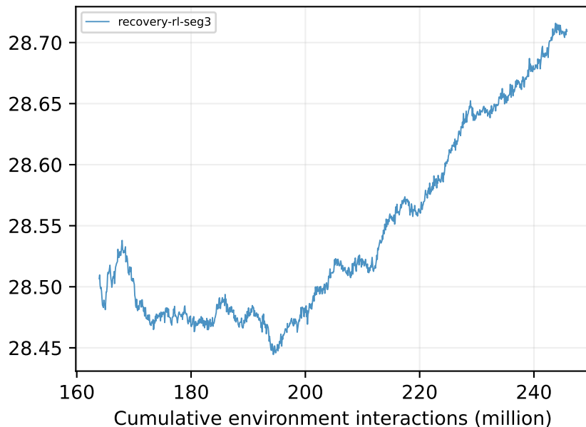
Actor loss
