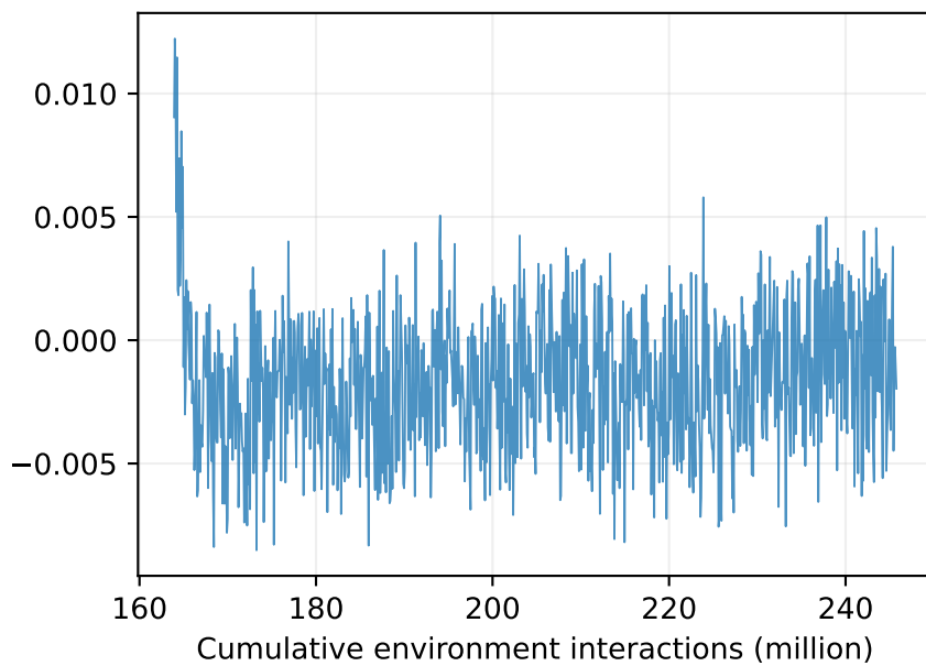
Actor loss
