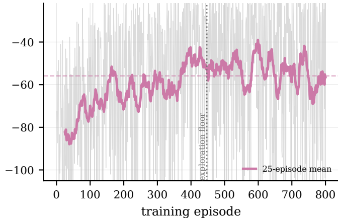
D evenness + in-vehicle cost (last 100 episodes: -55.9)
