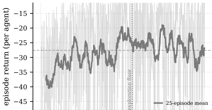
C both gaps vs schedule (last 100 episodes: -25.8)
