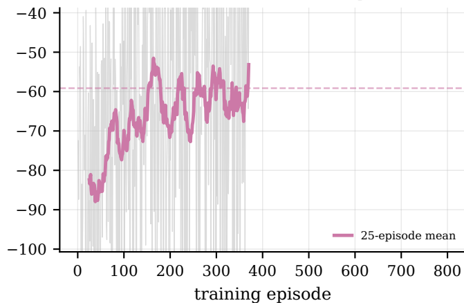
D evenness + in-vehicle cost (last 100 episodes: -59.1)
