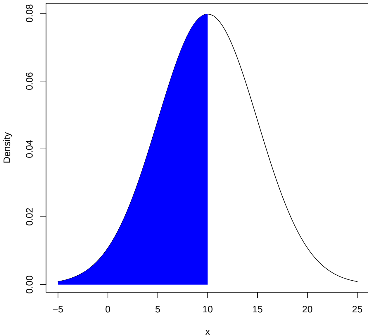
Normal Curve (mu = 10 , sigma = 5 )
