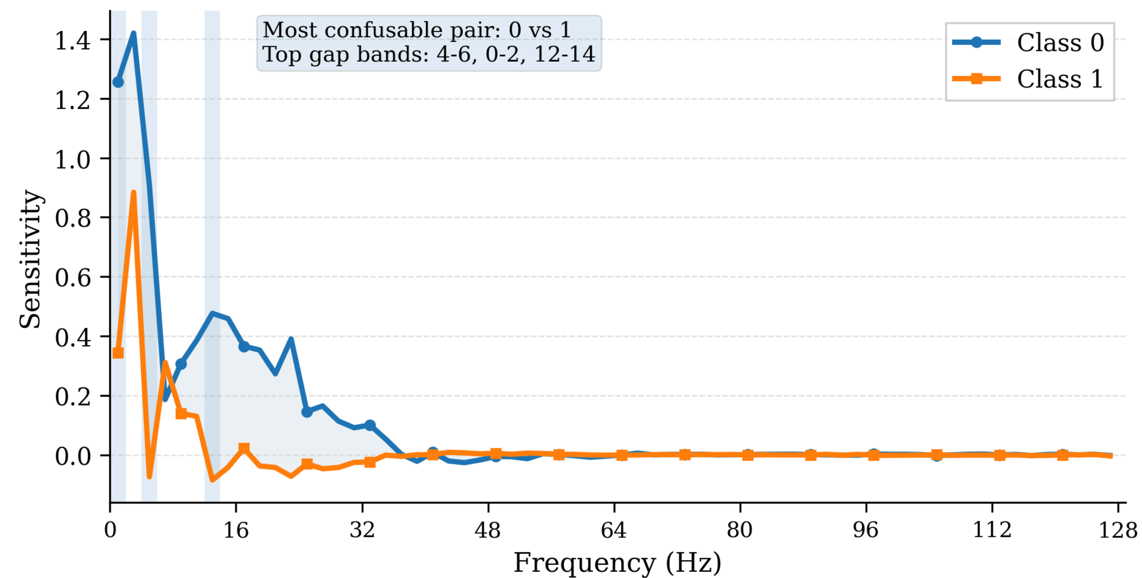
(e) PTB w/o SCLN
