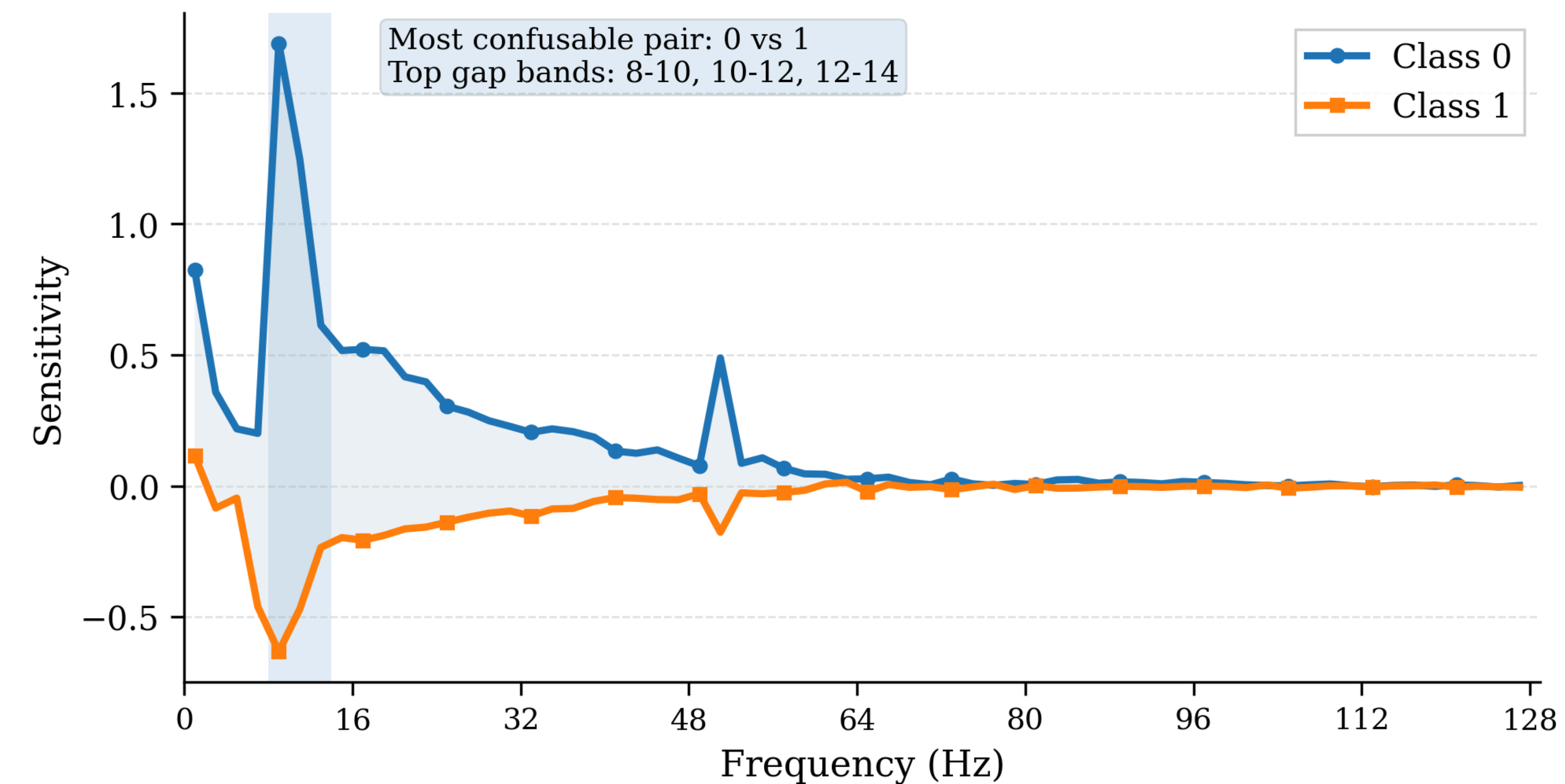
(c) APAVA w/ SCLN
