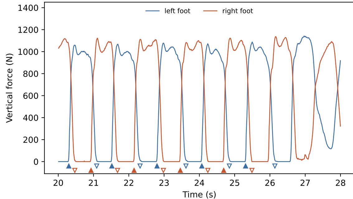
A. Total force per foot, record GaCo01_01; ▲ heel strike, ▼ toe off
