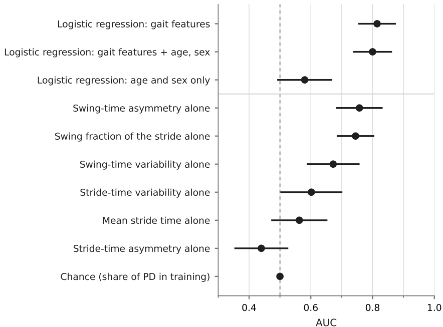
A Within protocol: participant-grouped 5-fold cross-validation, 20 repeats
