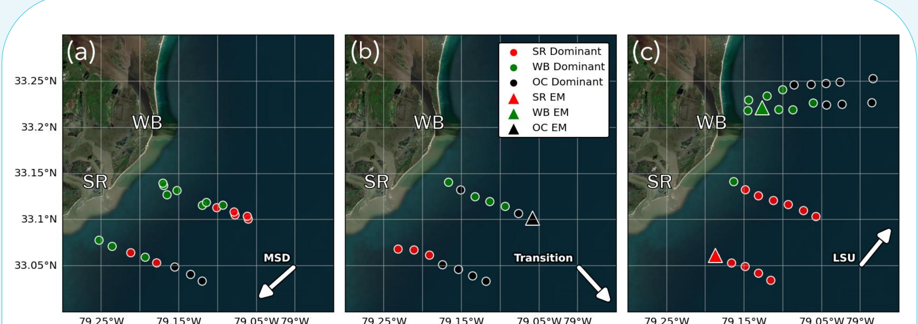
Figure 6. Geographic classification maps grouped by wind regime: (a) Medium Strength Downwelling (MSD), (b) Transition, and (c) Low Strength Upwelling (LSU). An arrow on each map shows the mean wind direction during that regime. Each station was classified by the endmember contributing its largest EMMA-derived fraction. The maps show how dominant Winyah Bay, Santee River, and ocean influence changed across the three wind regimes.
