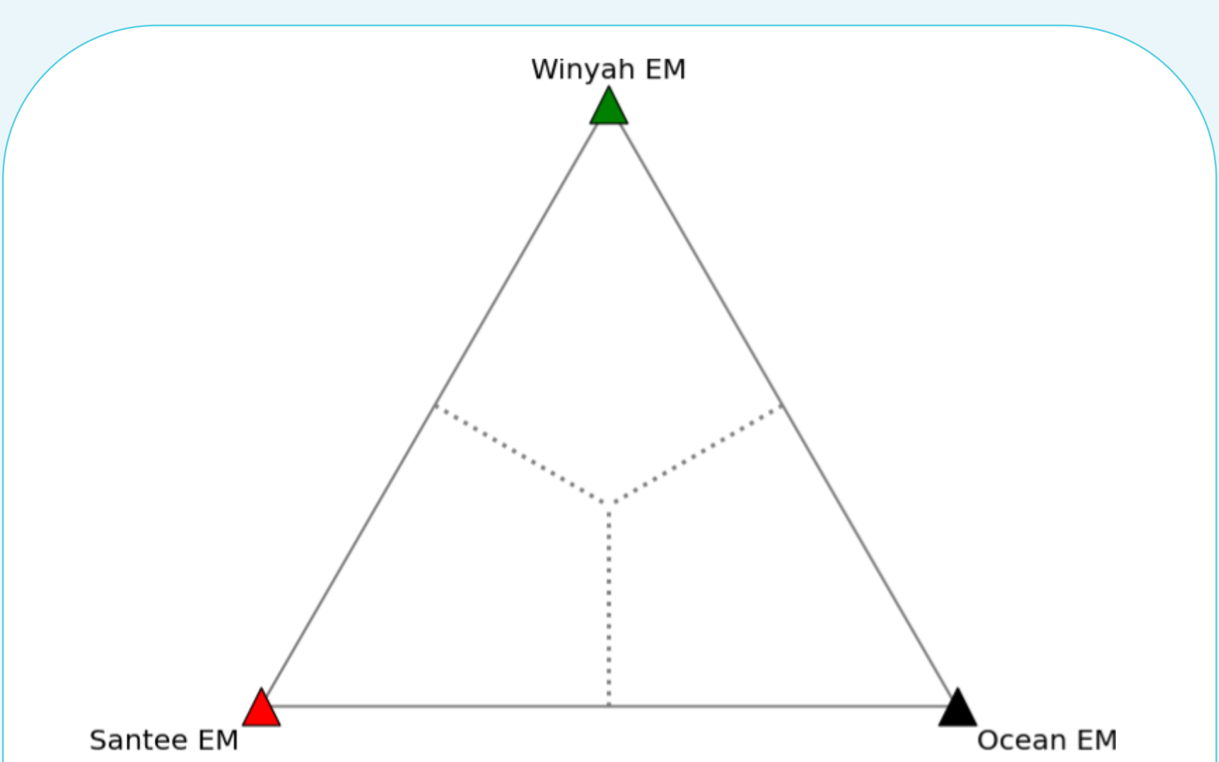
Figure 3. Ternary space for the three-endmember model. The vertices represent pure Winyah Bay, Santee River, and ocean endmembers. A station's position within the triangle is determined by its calculated source fractions; movement toward a vertex indicates increasing influence from that endmember.
