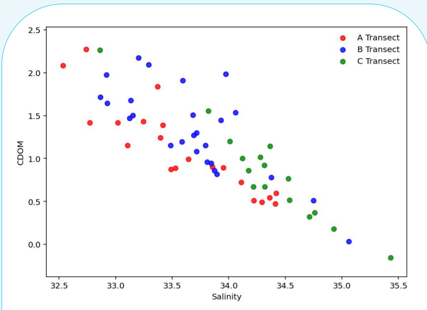
Figure 4. Plume-layer averaged salinity versus CDOM. This tracer pair shows the clearest structure and grouping, but transects still overlap, motivating a mixing analysis rather than a simple visualization.
