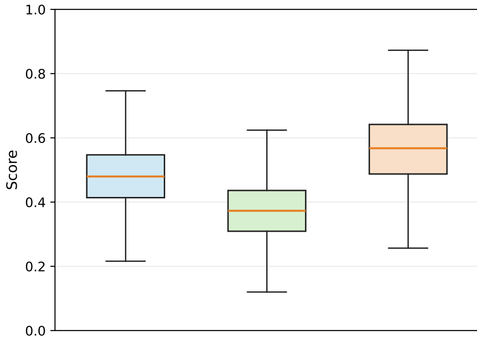
Sentence-transformer cosine
